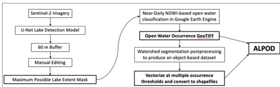
Figure 2. Methodological approach to constructing the ALPOD dataset.
