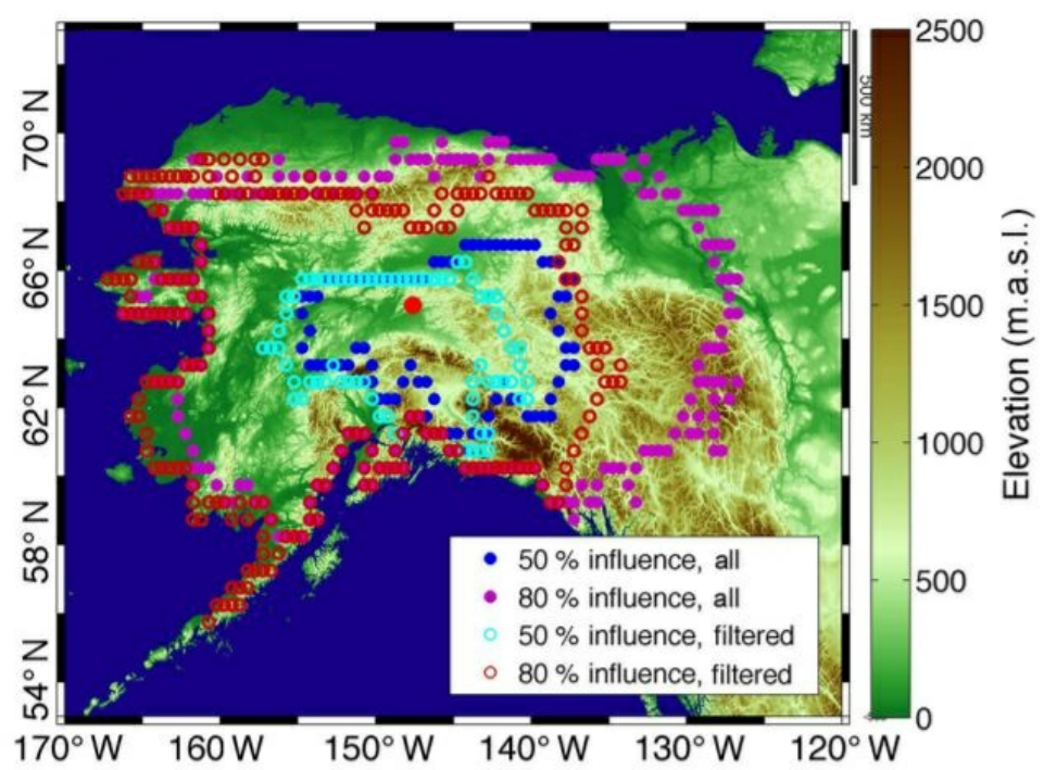
Figure 1. Surface contours (50% --- blue; 80% --- purple) for the average WRF-STILT influence functions (mid-afternoon averages 2012-2014) show CO 2 and CH 4 measurements from the CARVE tower have a high sensitivity to the boreal forests and lowlands of interior Alaska. Cyan and red circles are shown for the footprints after filtering (from Karion et al., 2016).
