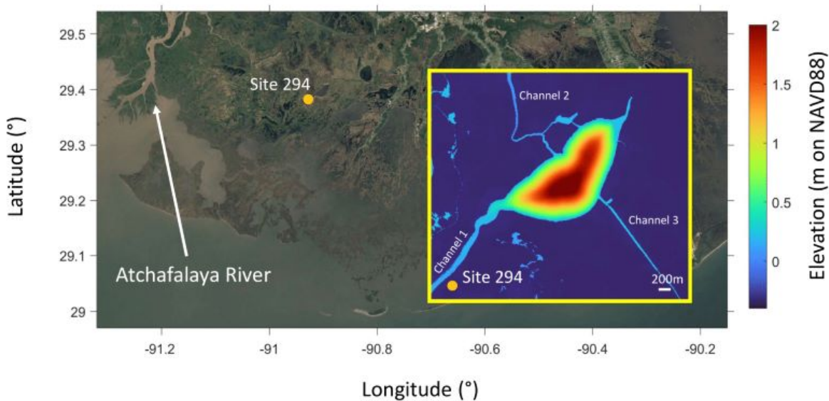
Figure 1. Satellite image of Terrebonne Bay, Louisiana, USA with location of Site 294. Inset shows bathymetry of this intensive site.
