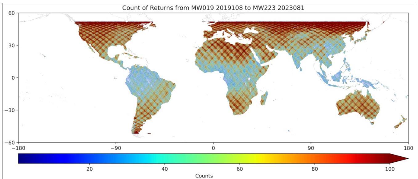
Figure 6. Count of valid laser footprints per grid cell. Image derived from dataset file GEDI03_counts_2019108_2023081_002_05.tif.
