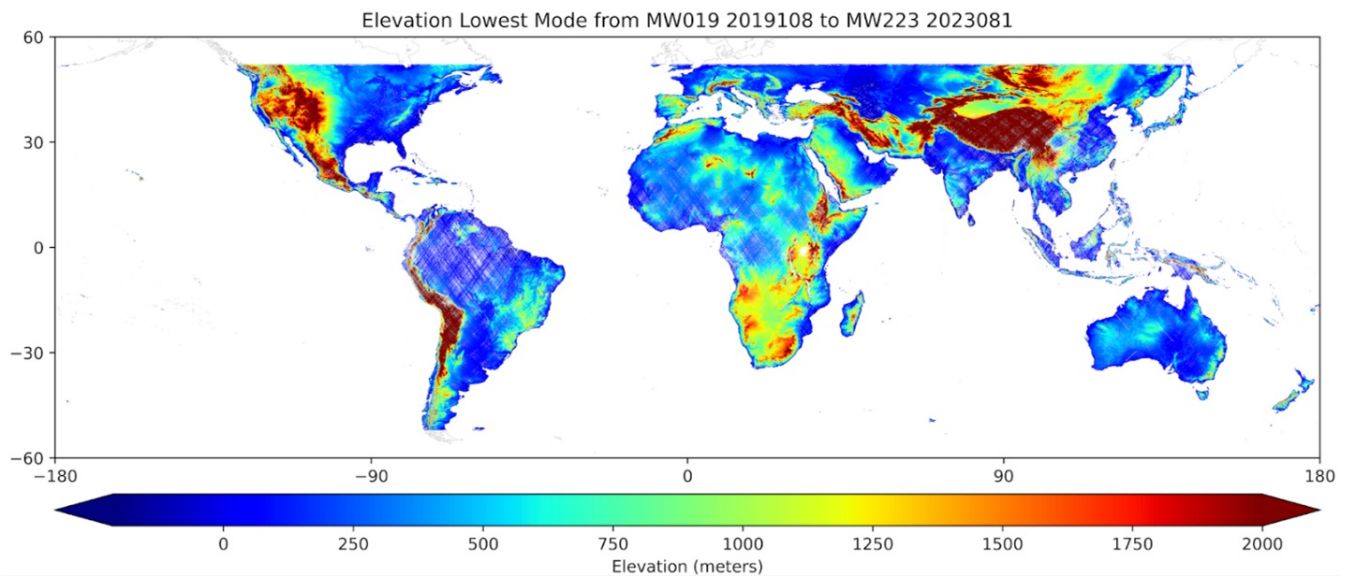
Figure 4. Estimated mean elevation of lowest mode. Image derived from the dataset file GEDI03_elev_lowestmode_mean_2019108_2023081_002_05.tif.
