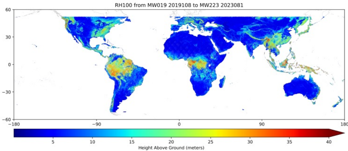
Figure 1. Level 3 estimated canopy height in meters derived from the Level 2 profile metric RH100 between the 19th and the 223rd mission week. Source: GEDI03_rh100_mean_2019108_2023081_002_05.tif
